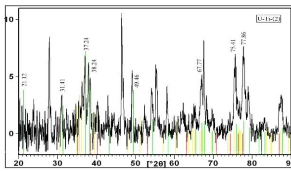
Figure 5.6: The X-ray diffraction spectra of the U-Ti-(2) alloy with 2\theta for the maxima of the U_2Ti compound
