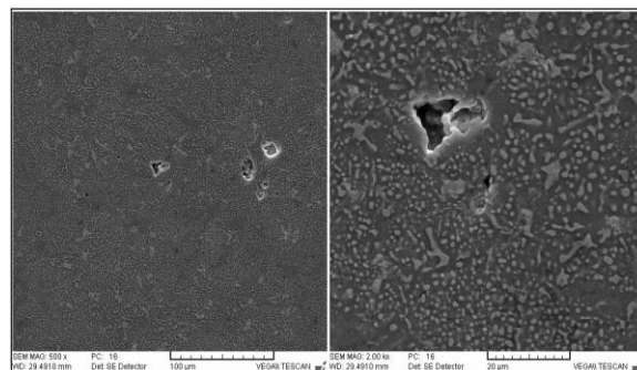
Figure 4.70: The morphology of the U-55Zr-H compound, after 100 thermal cycles
