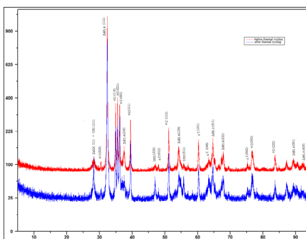
Figure 4.71: The diffraction spectra before and after 100 thermal cycles
