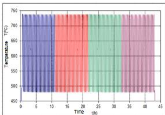
Figure 4.66: The temperature variation for 100 heating / cooling cycles on the \text{U-ZrH}_{1.6} compound
