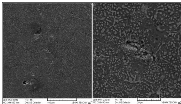
Figure 4.69: The morphology of the U-55Zr-H compound, before the thermal cycles
