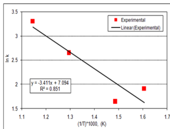
Figure 5.26: Arrhenius plot for activation energy calculation, stage II
