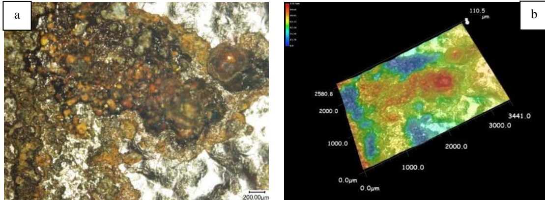
Fig.10 2D (a) and 3D (b) micrographs of the metal surface in "6 o'clock" position, monitoring campaign 7, 100X
