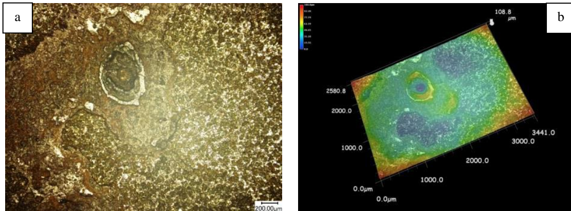
Fig.11 2D (a) and 3D (b) micrographs of the metal surface in "6 o'clock" position, monitoring campaign 2, 100X
