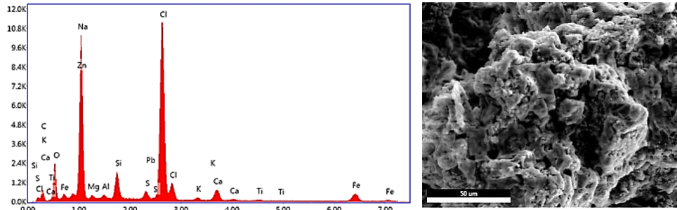
Fig.9 EDS spectrum of the deposit and SEM micrograph of sample from which spectrum was generated
