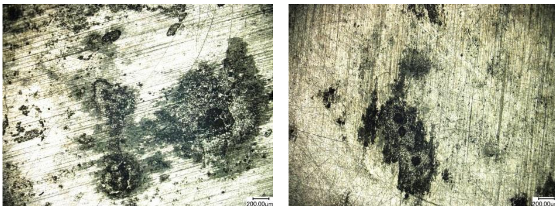
Fig.12 2D micrographs of the metal surface in "12 o'clock" position, monitoring campaign 3, 100X
