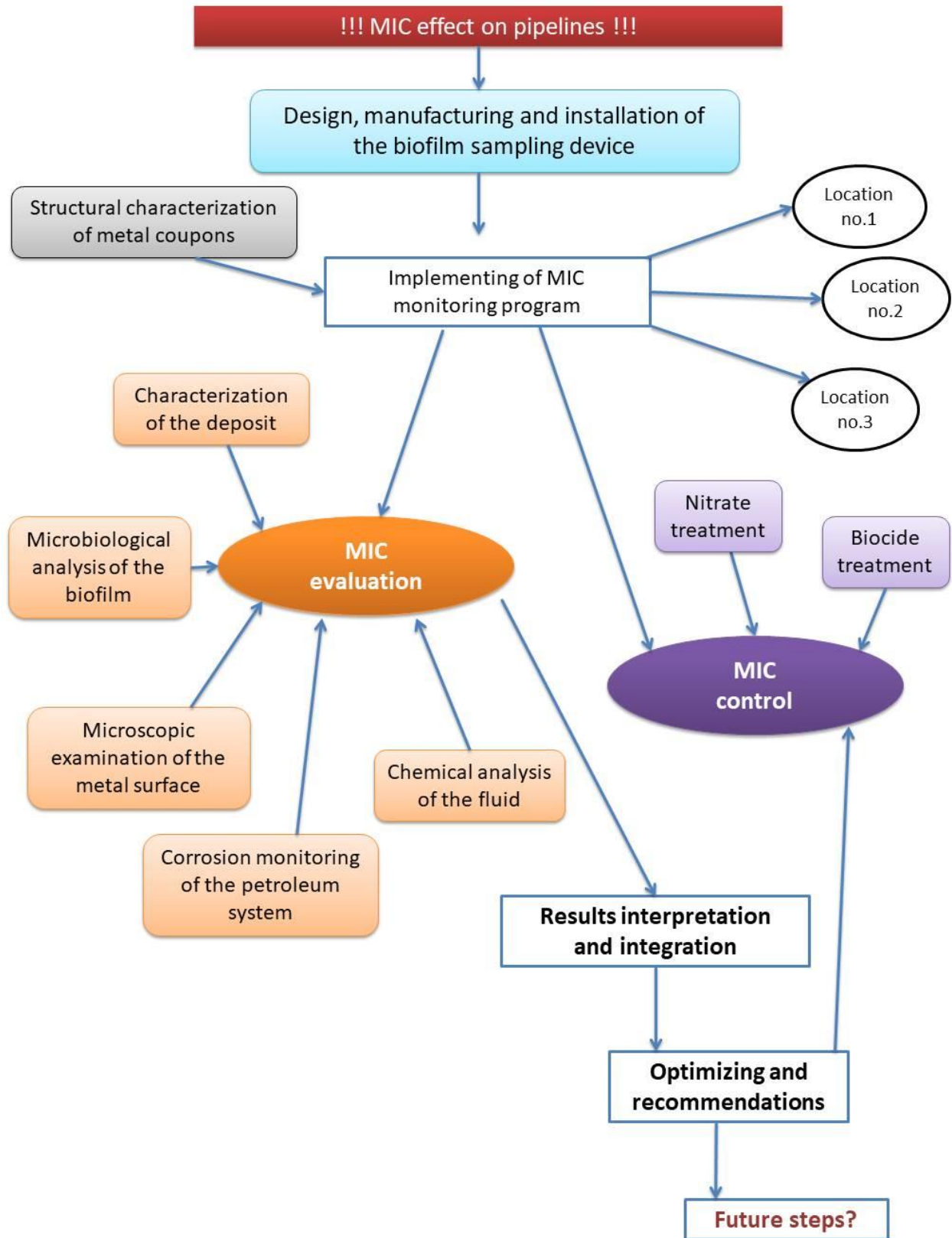
Fig.8 The experimental program of the research carried out within the present PhD thesis
